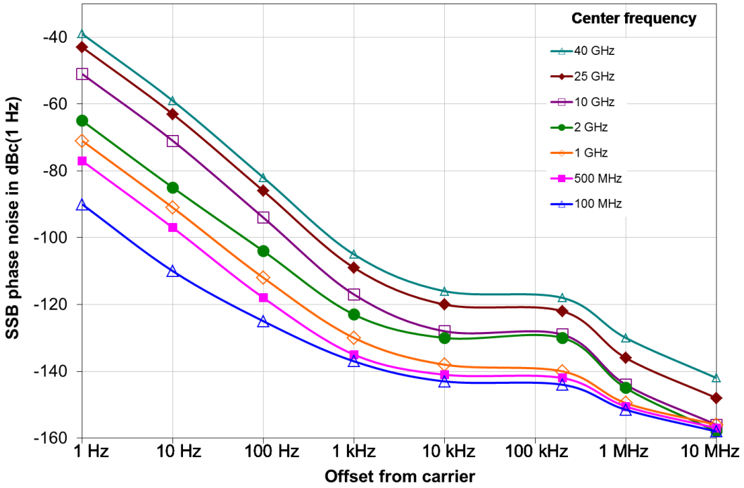
Typical phase noise at different center frequencies (with the R&S®ESW-B4 option for offsets ≤ 10 Hz)
